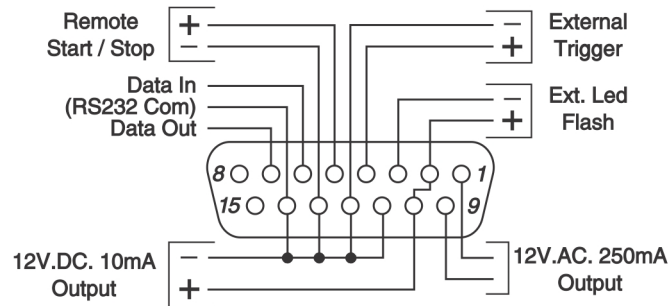
15 Pin Socket on Stroboscope Front Panel
